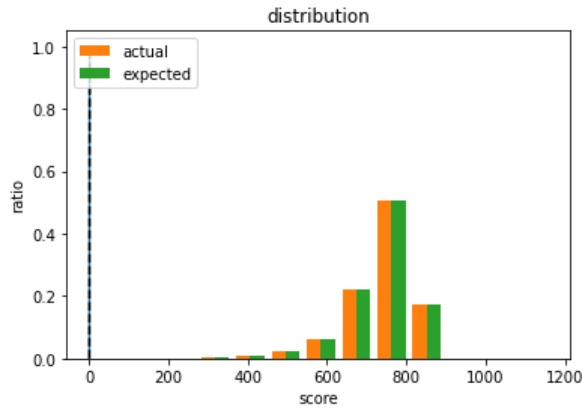
Fig . 11 PSI Chart of LR-WOE Model
