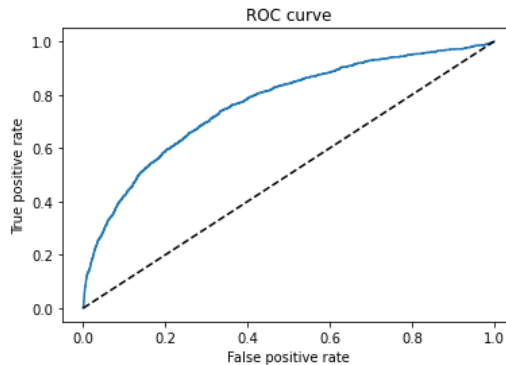
Fig. 1 ROC Curve of the LR Model
