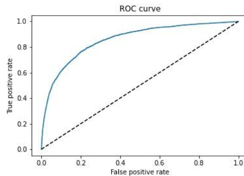
Fig. 6 ROC Curve of the LR-WOE Model
