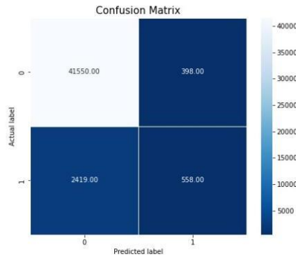
Fig. 5 Confusion Matrix of the LR-WOE Model
