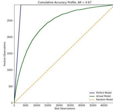
Fig. 10 CAP of the LR-WOE Model After Feature Selection
