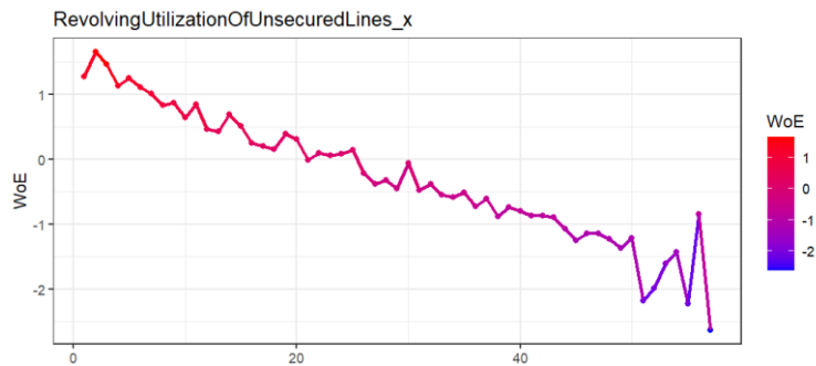
Fig. 3 WOE Encoding Values Chart of Available Credit Ratio
