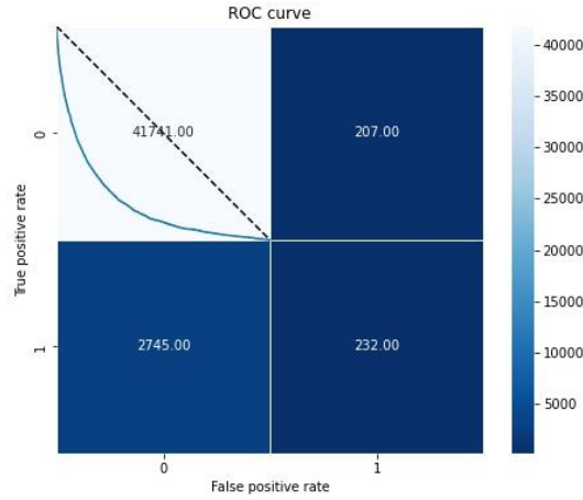
Fig. 8 Confusion Matrix and ROC Curve of the LR-WOE Model After Feature Selection
