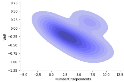
Fig. 2 WOE Encoding Values Chart of Number of Dependents
