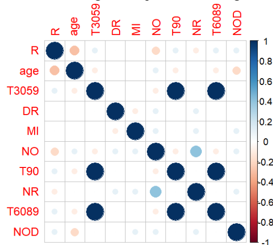
Fig. 7 Feature Heatmap
