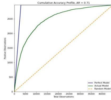
Fig. 9 CAP Chart of the LR-WOE Model
